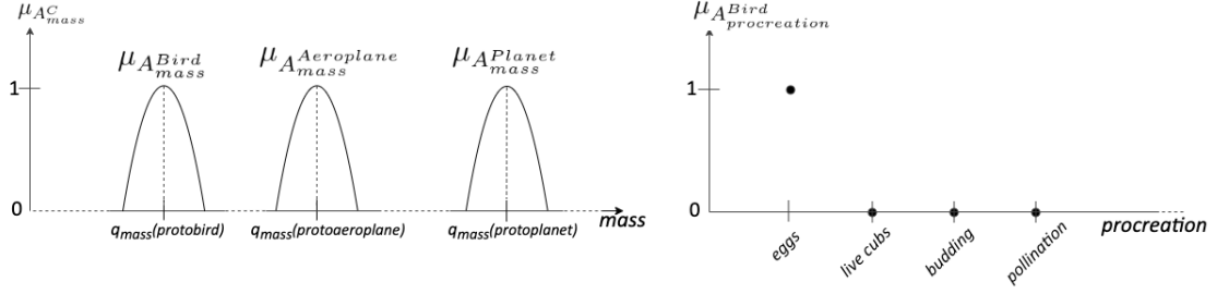
Figure 1: Left: Illustration of the membership functions \mu for a continuous quality dimension mass across three example concepts. Prototypical instances are assumed to bear prototypical value of the property. Right: Illustration of a nominal quality dimension procreation for the Bird concept.
